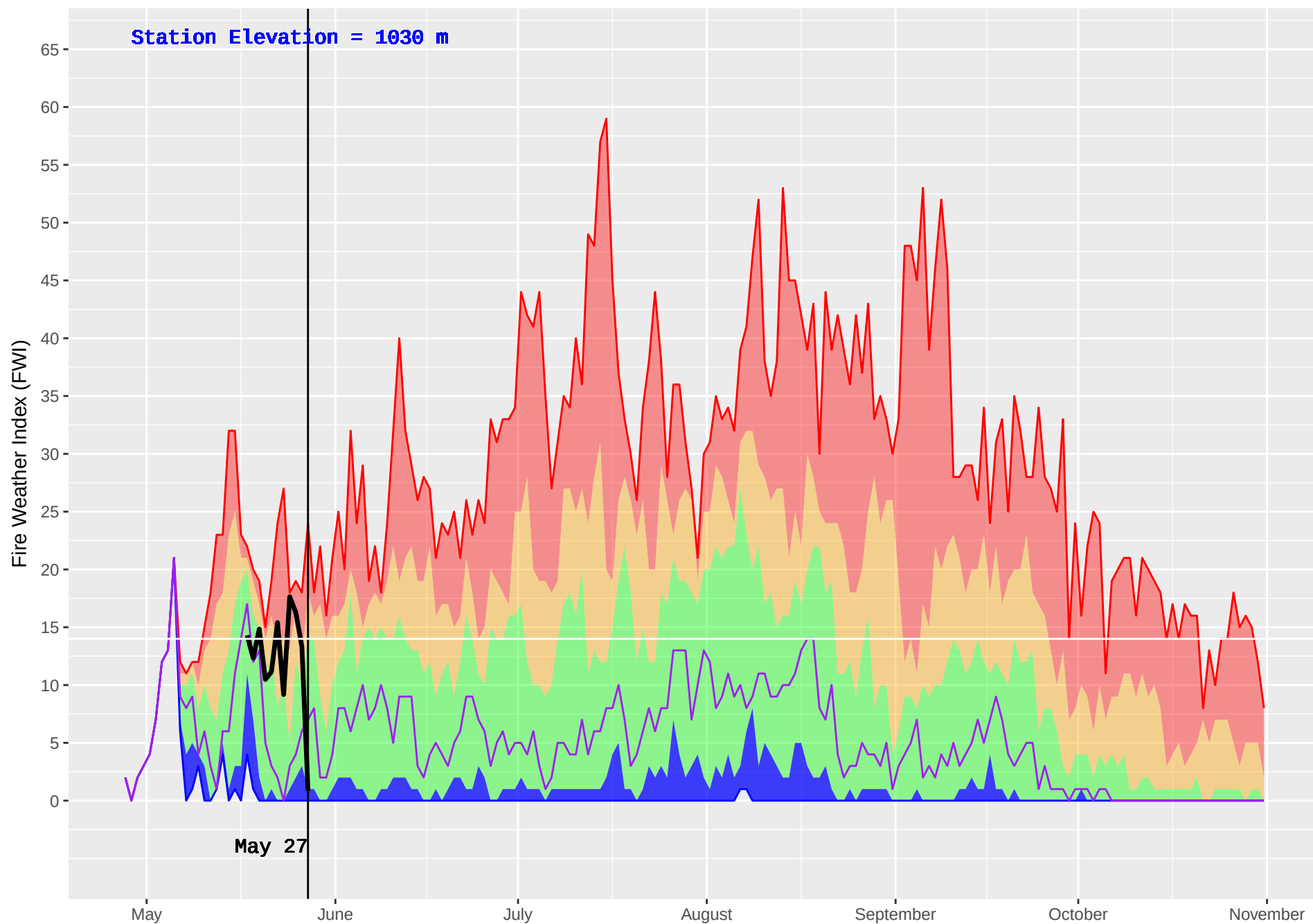
WITCH (154) : Historical (1993–2016) and Current (2018) Noon Fire Weather Index (FWI)
