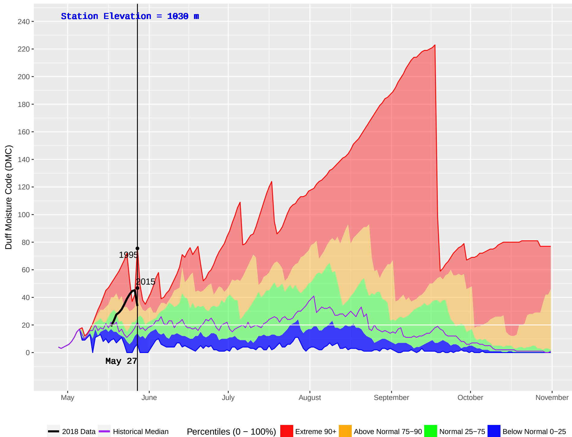
WITCH (154) : Historical (1993–2016) and Current (2018) Noon Duff Moisture Code (DMC)
