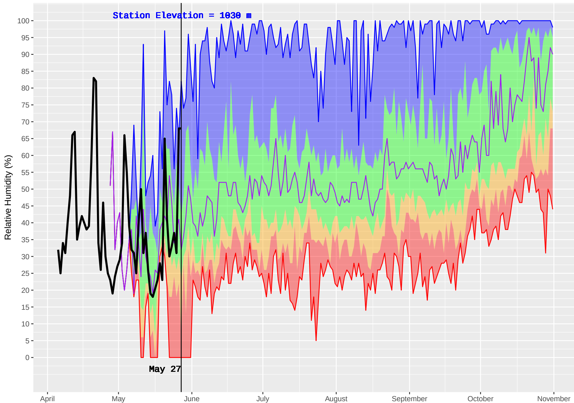
WITCH (154) : Historical (1993–2016) and Current (2018) Noon Relative Humidity
