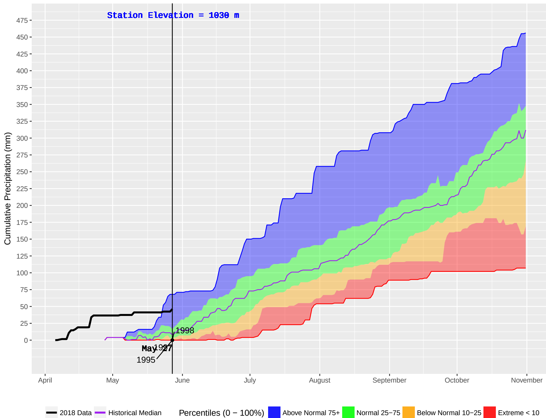
WITCH (154) : Historical (1993–2016) and Current (2018) Noon Cumulative Precipitation
