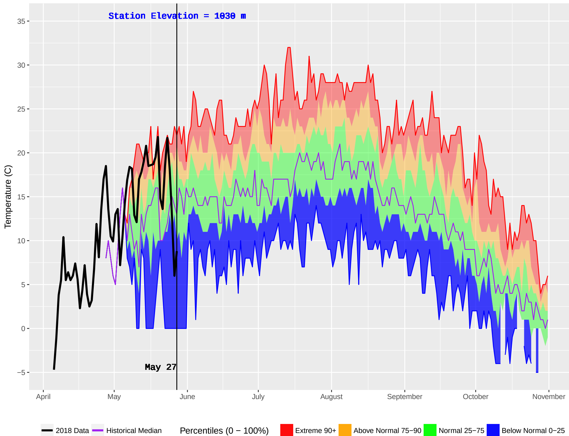
WITCH (154) : Historical (1993–2016) and Current (2018) Noon Temperature
