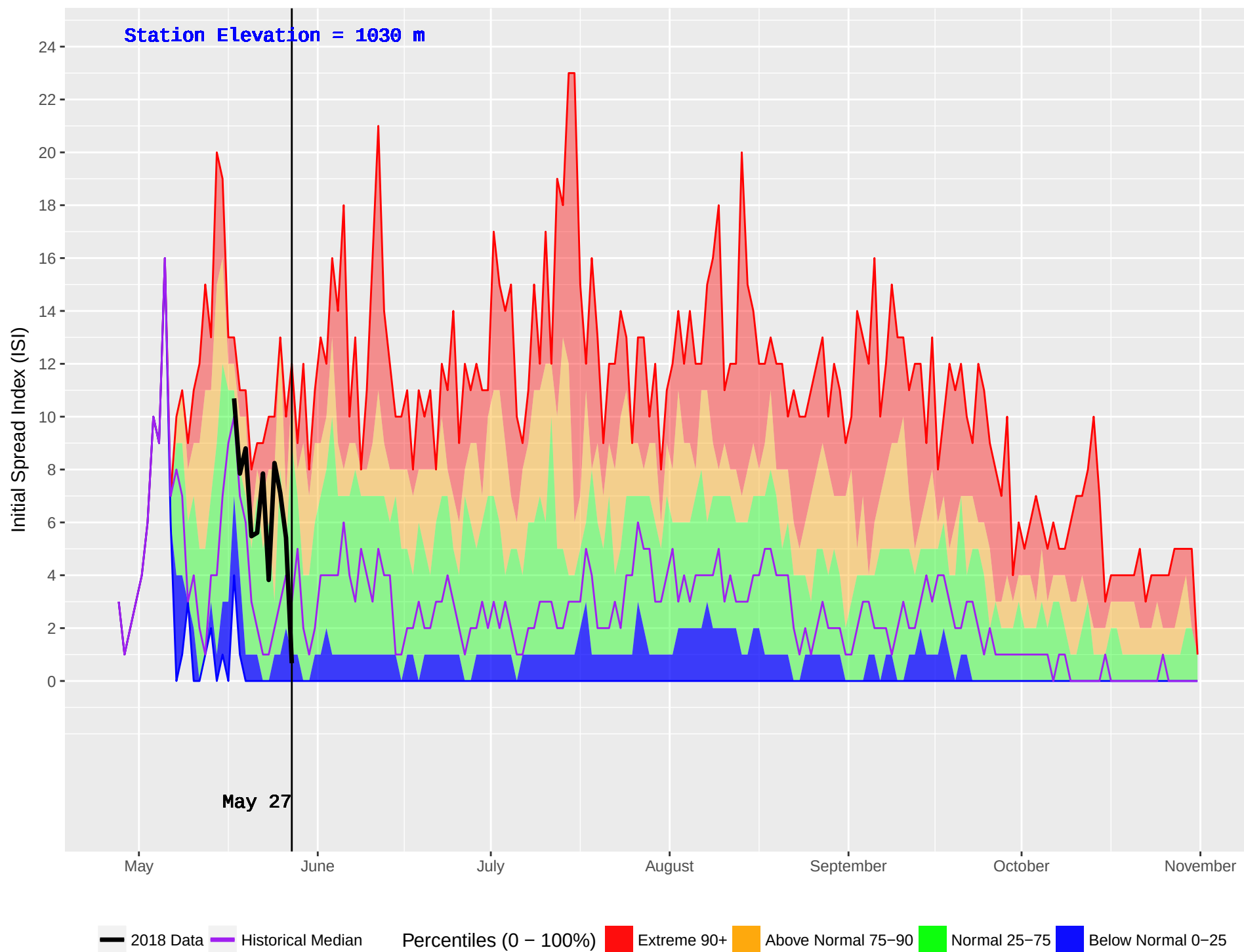
WITCH (154) : Historical (1993–2016) and Current (2018) Noon Initial Spread Index (ISI)
