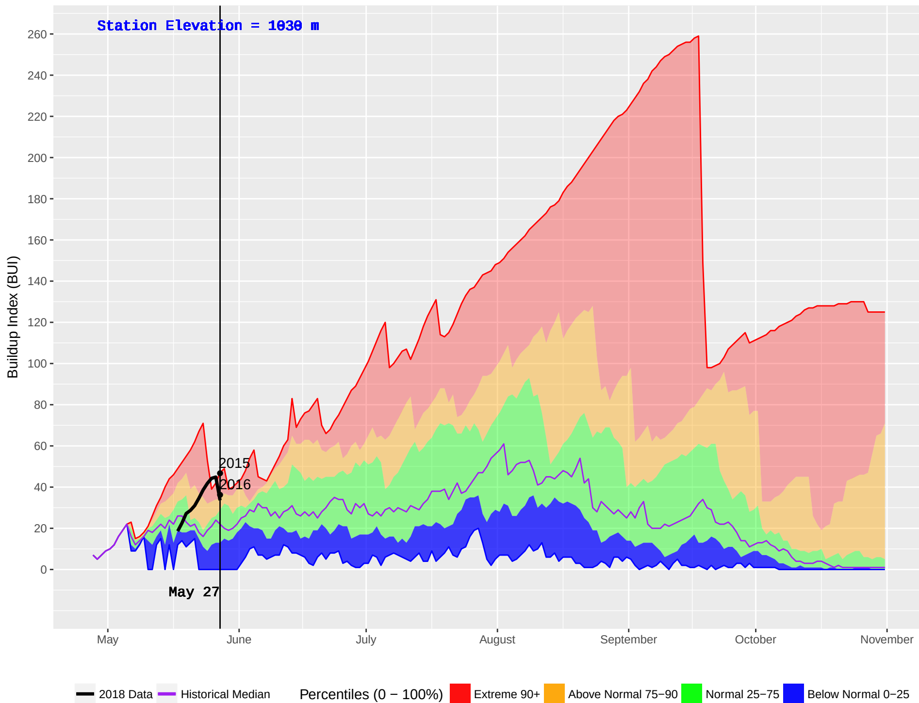
WITCH (154) : Historical (1993–2016) and Current (2018) Noon Buildup Index (BUI)
