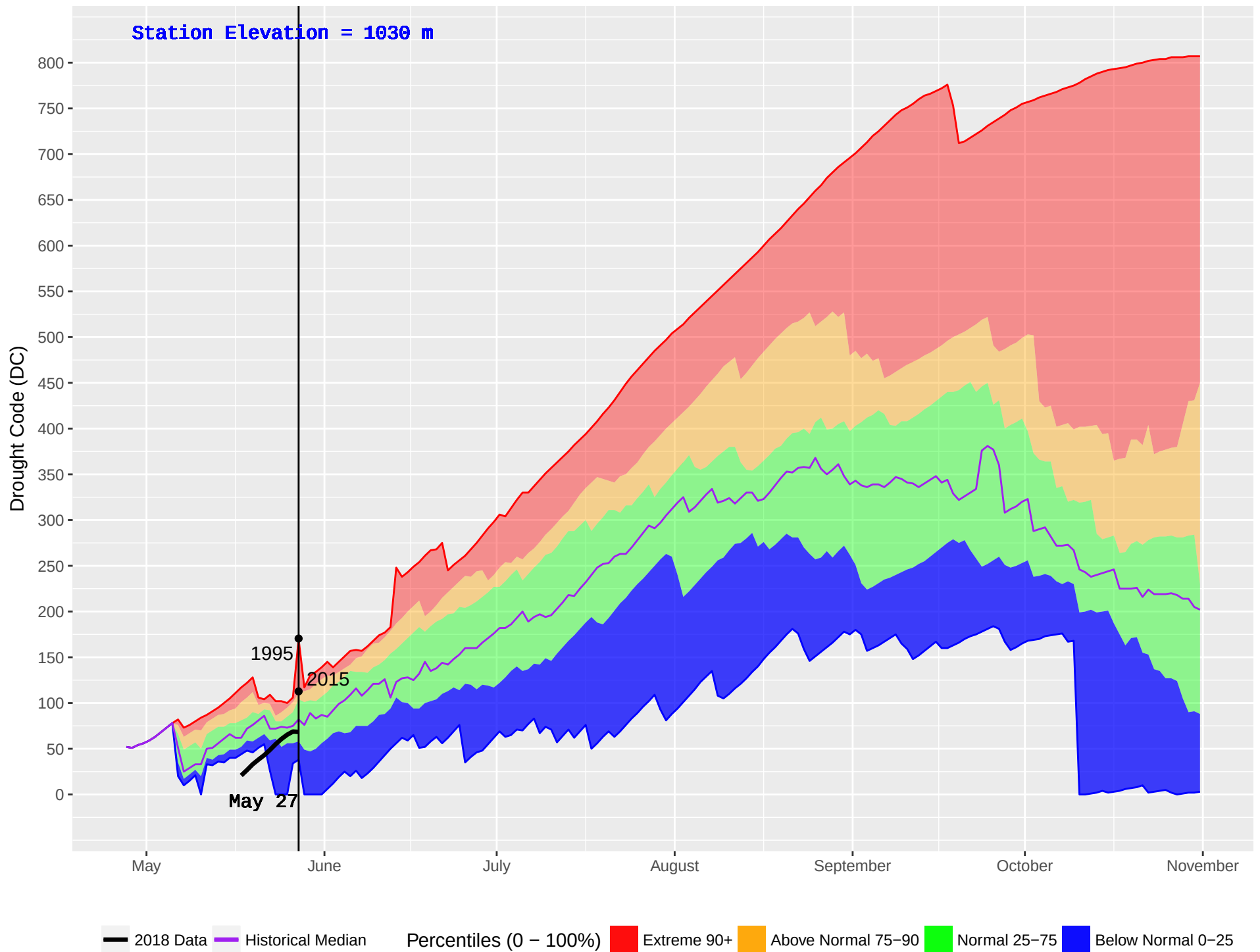
WITCH (154) : Historical (1993–2016) and Current (2018) Noon Drought Code (DC)
